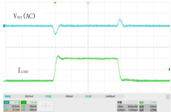
图 23. 负载瞬态响应, V_{IN}=4.3V , V_{OUT}=3.3V , I_{OUT}=1mA to 150mA
