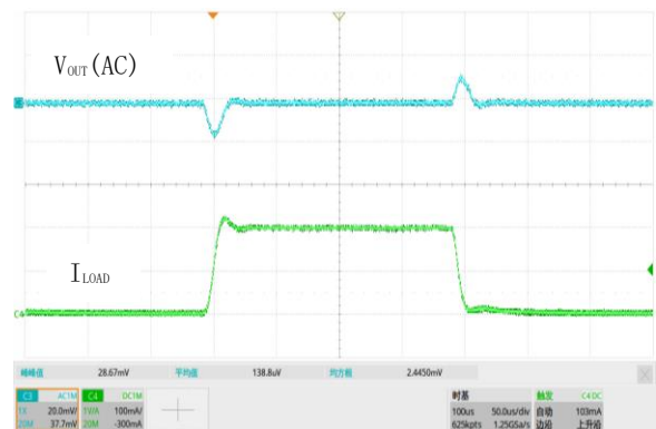
图 24. 负载瞬态响应, V_{IN}=4.3V , V_{OUT}=3.3V , I_{OUT}=1mA to 200mA
