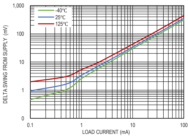
图 9. Output Swing V_{OH} vs. Load Current, V_S = \pm 2.5V
