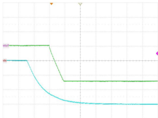
图 19. 软启动, V_{IN} = -6V , V_{OUT} = -5V , I_O = -200mA
