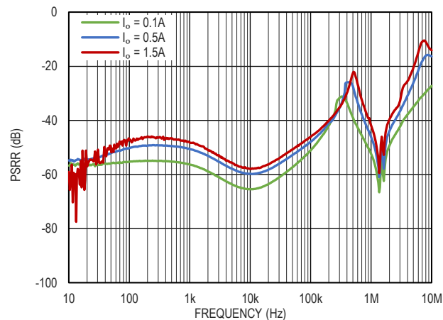
图 21. PSRR, V_{IN} = 5.3V , V_{OUT} = 5.0V
