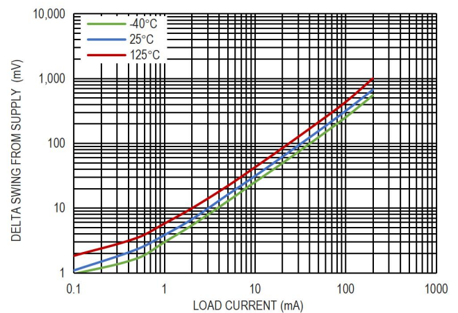
图 10. Output Swing V_{OL} vs. Load Current, V_S = \pm 2.5V
