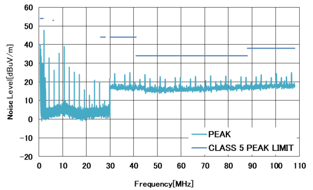
图 33. GM2500_DEMOZ CISPR25 Conducted Emission with Class 5 Peak Limits (Voltage Method)
