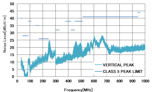
图 35. GM2500_DEMOZ CISPR25 Radiated Emission (Vertical)
