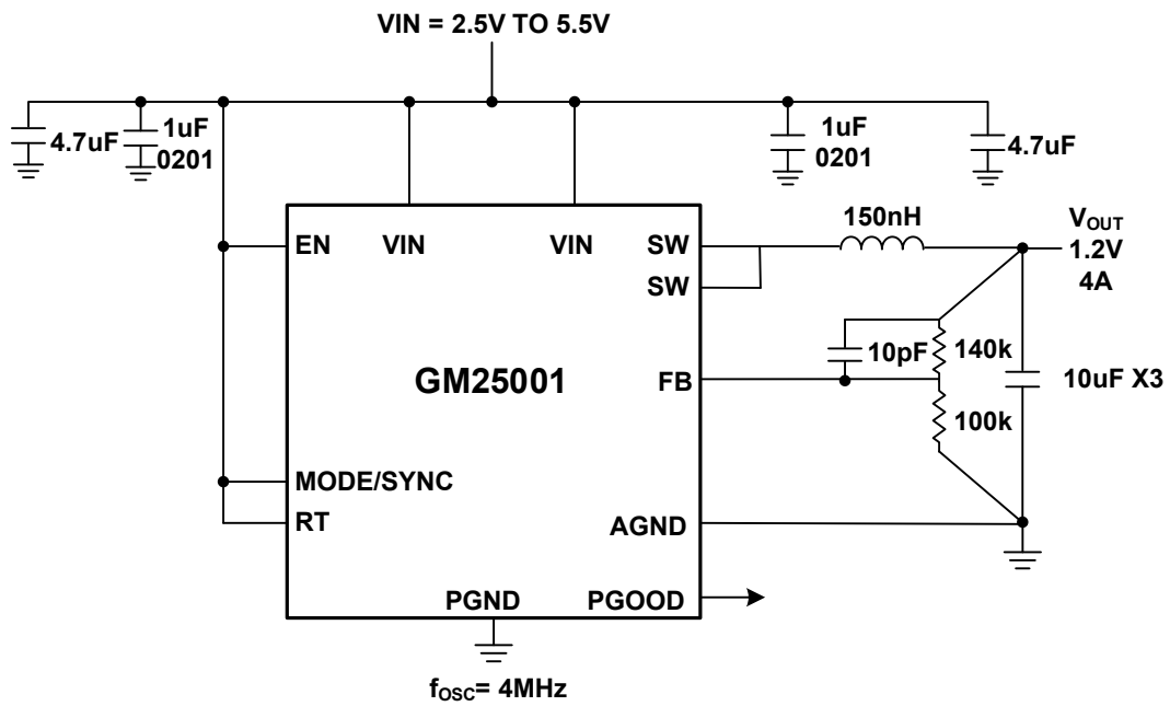
图 37. 4MHz, V IN =3.3V, V OUT =1.2V, I LOAD =4A
