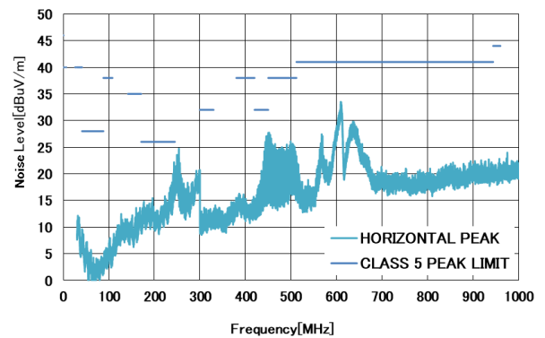
图 34. GM2500_DEMOZ CISPR25 Radiated Emission (Horizontal)
