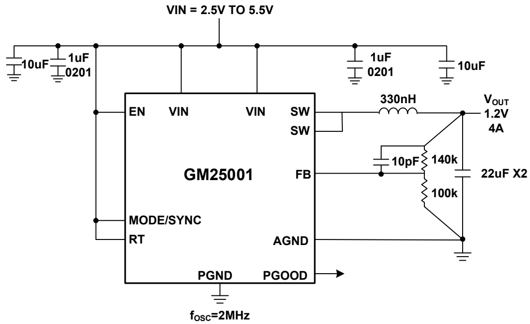
图 36. 2MHz, V IN =3.3V, V OUT =1.2V, I LOAD =4A
