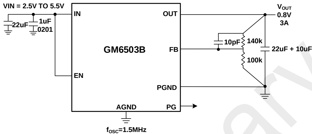
图 17. V IN =3.3V, V OUT =0.8V, I LOAD =3A
