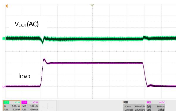
图 22. 负载瞬态响应, V_{IN}=4.3V , V_{OUT}=3.6V , I_{OUT}=5mA to 200mA
