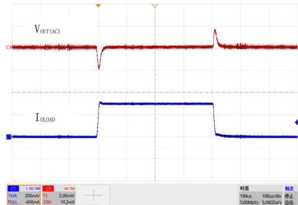
图 20. 负载瞬态响应, V_{IN}=4.3V , V_{OUT}=3.3V , I_{OUT}=1mA to 300mA
