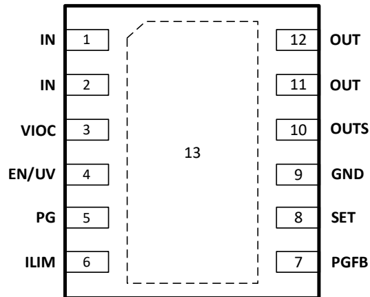
图 6. DFN12(4mmx4.9mm GM12051ACPZ-1 兼容 MSOP-12 和 3mmx3mm GM12051ACPZ-4)引脚配置(顶视图)
