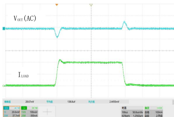
图 25. 负载瞬态响应, V_{IN}=4.3V , V_{OUT}=3.3V , I_{OUT}=1mA to 200mA
