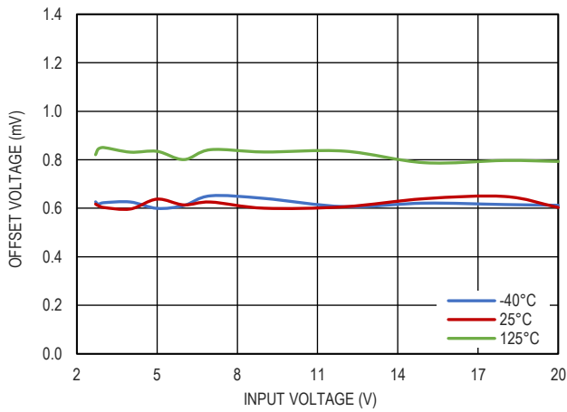
图 5. |V OUT -V SET |和输入电压的关系, V OUT =3.0V
