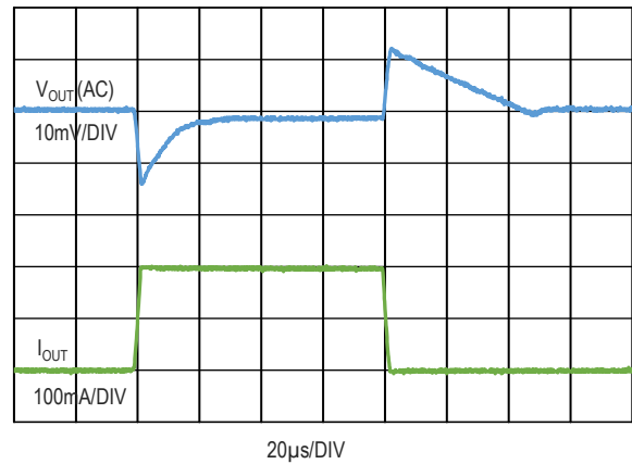
图 20. 负载瞬态响应, V_{IN}=4V , V_{OUT}=3.3V , I_{OUT}=1mA to 200mA
